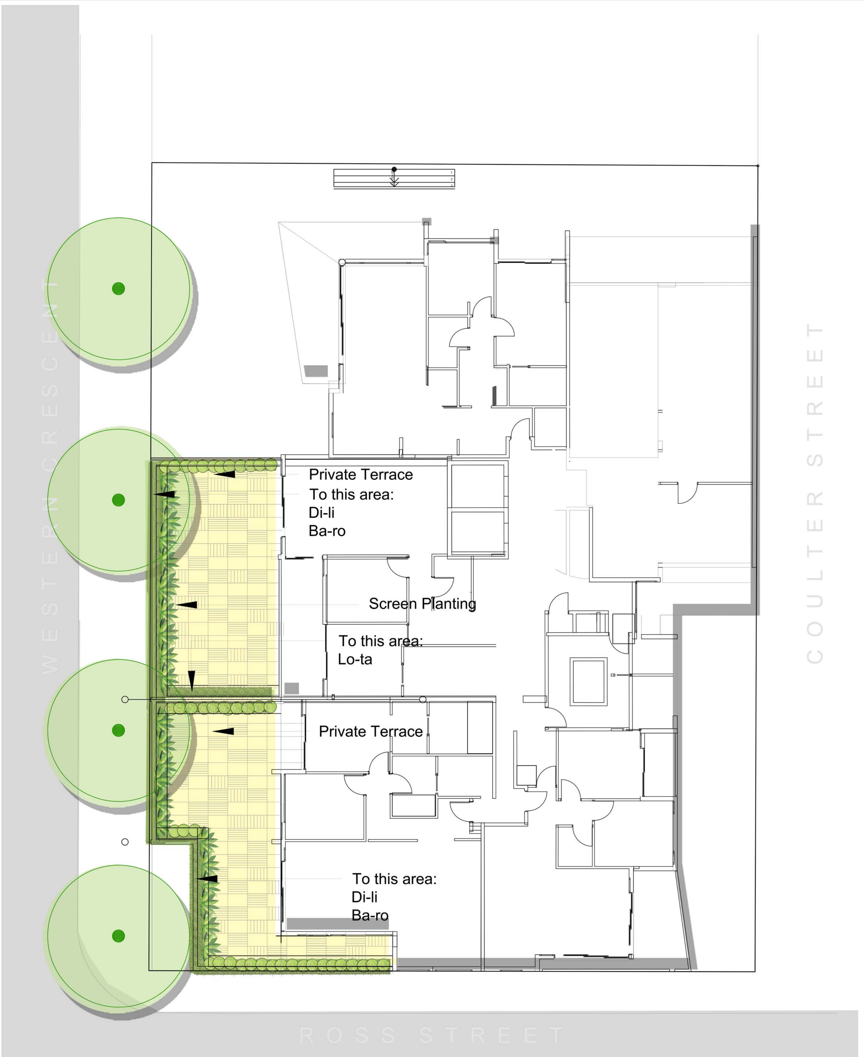
LEVEL TWO LANDSCAPE PLAN
